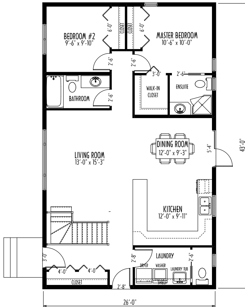
MAIN FLOOR PLAN 1118 SQ. FT.
