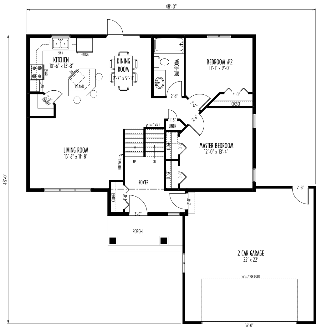
MAIN FLOOR PLAN AREA: 1041 sq. ft.
